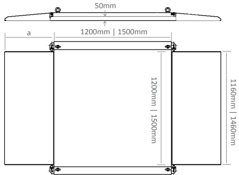
a = default of 300mm ramp, optional 500mm
