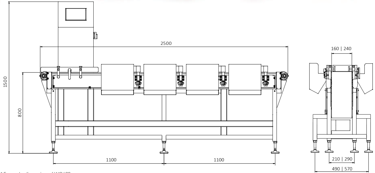
* Example dimension of WG600 * Dimension in mm
