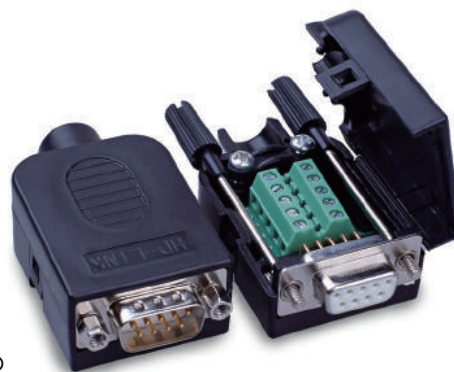
DB9P
