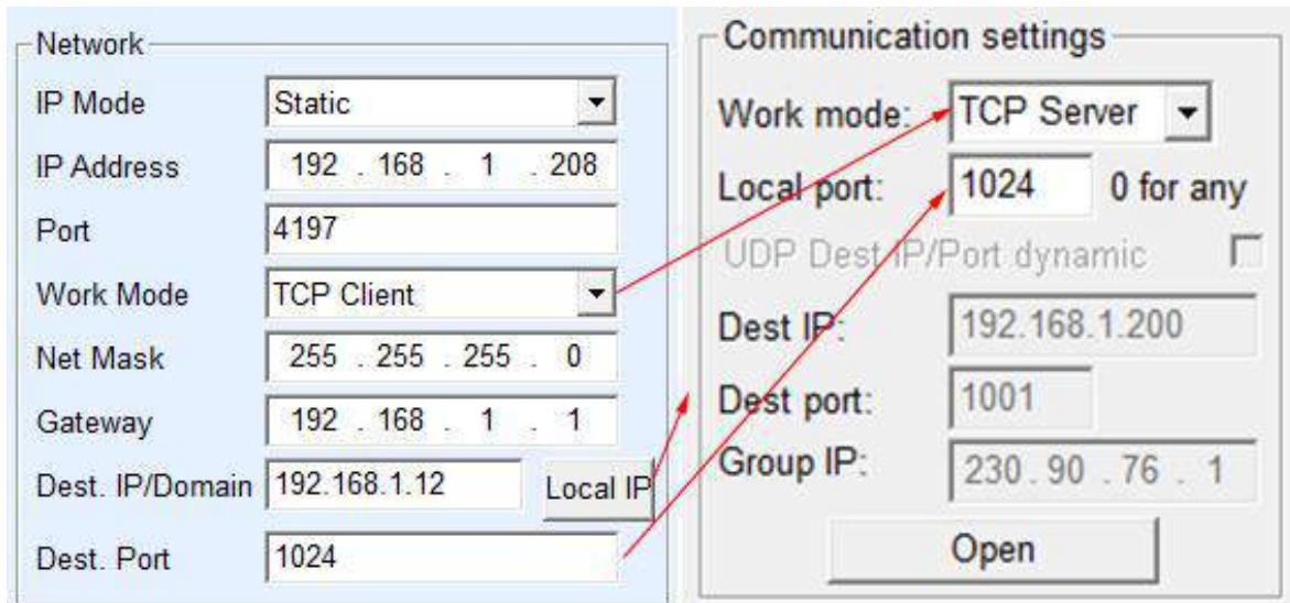
Figure 29 Networking Products as Client
