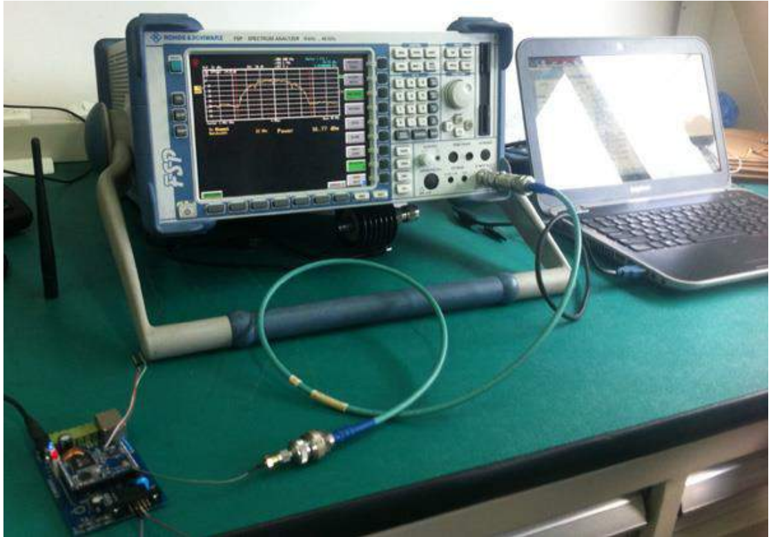
Figure 10 7104 Signal Test
