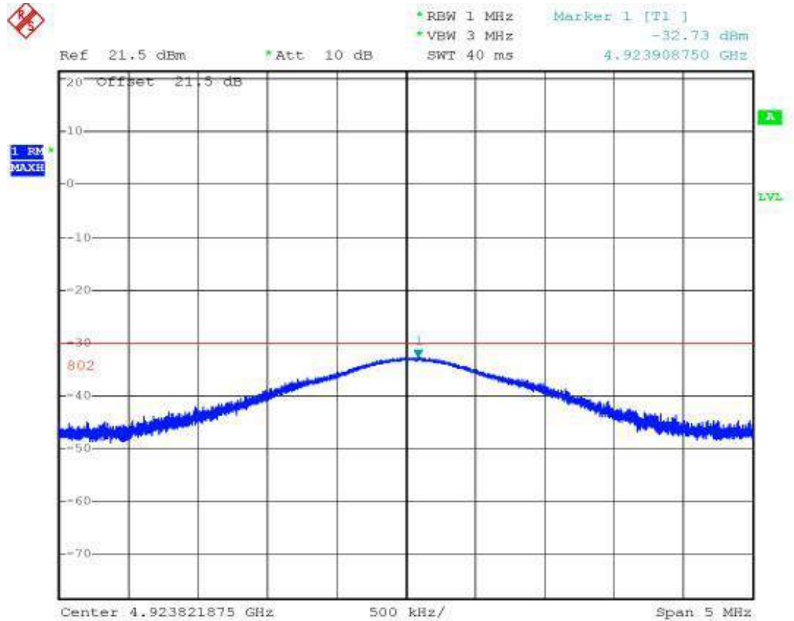
Figure 13 7104 Stray Test Curve
