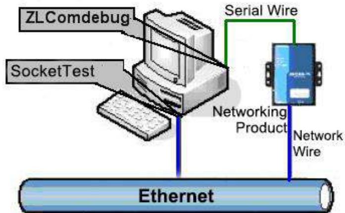
Figure 21 Transparent Transmission Diagram
