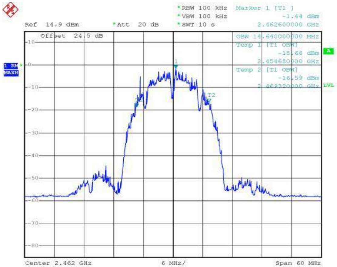
Figure 11 7104 Bandwidth Test Curve
