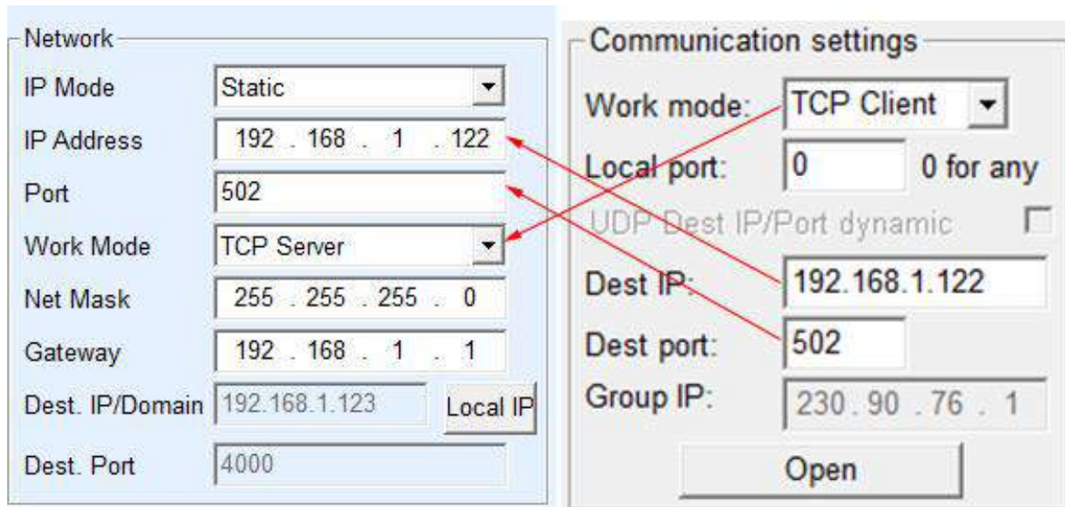
Figure 30 Networking Products as Server
