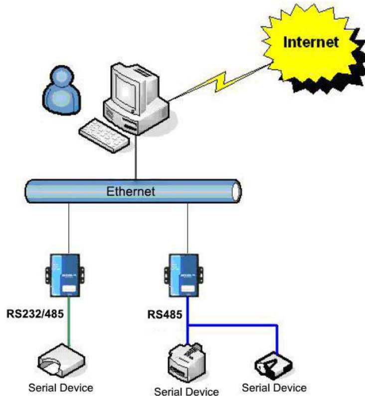
Figure 2 RWiFi Network Structure
